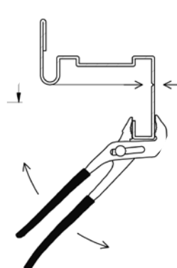
Lower Profile Profilo inferiore
